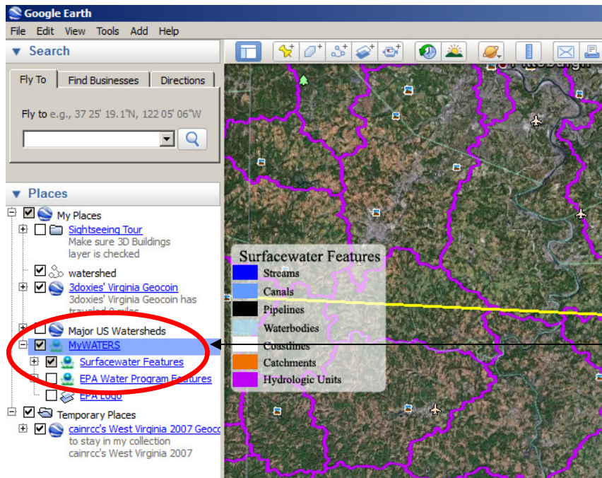
Figure 4. Using the MyWATERS menu. (Screenshot © 2012 Google Earth).
