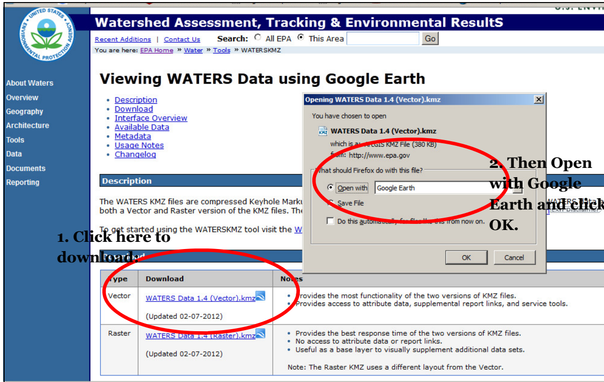
Figure 3. Downloading EPA WATERS data for viewing in Google Earth.
