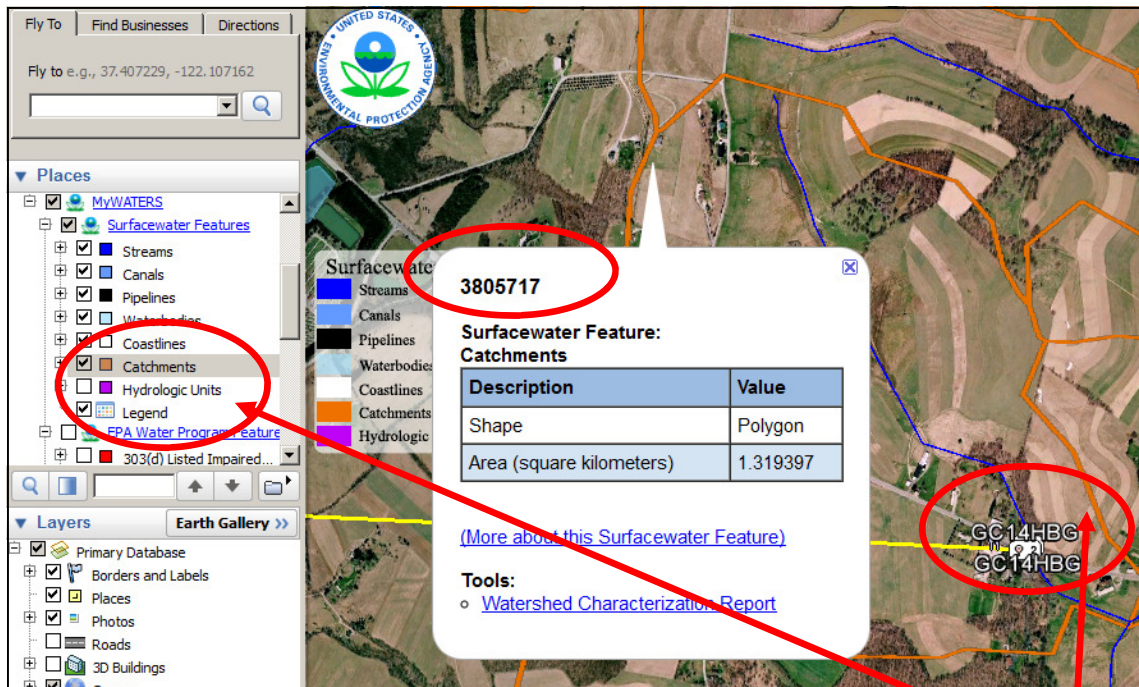
Figure 5. To learn more about the catchment that contains your farm site, uncheck the Hydrologic Units menu item. Click anywhere inside the orange catchment boundary that surrounds your farm site (Geocache site) to bring up the pop-up information box. The title at the top of the box is the name or number of the catchment, and the box also contains the catchment area. (Screenshot © 2012 Google Earth).
