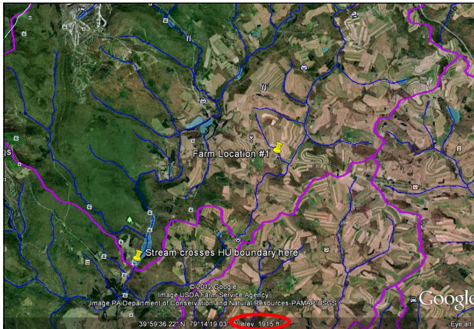
Figure 8. Placemarks added to the farm site and outlet point of the Hydrologic Unit containing the farm site. To read elevation at a point, hover your mouse over the point and look at the bottom of the map panel (circled in red above).
